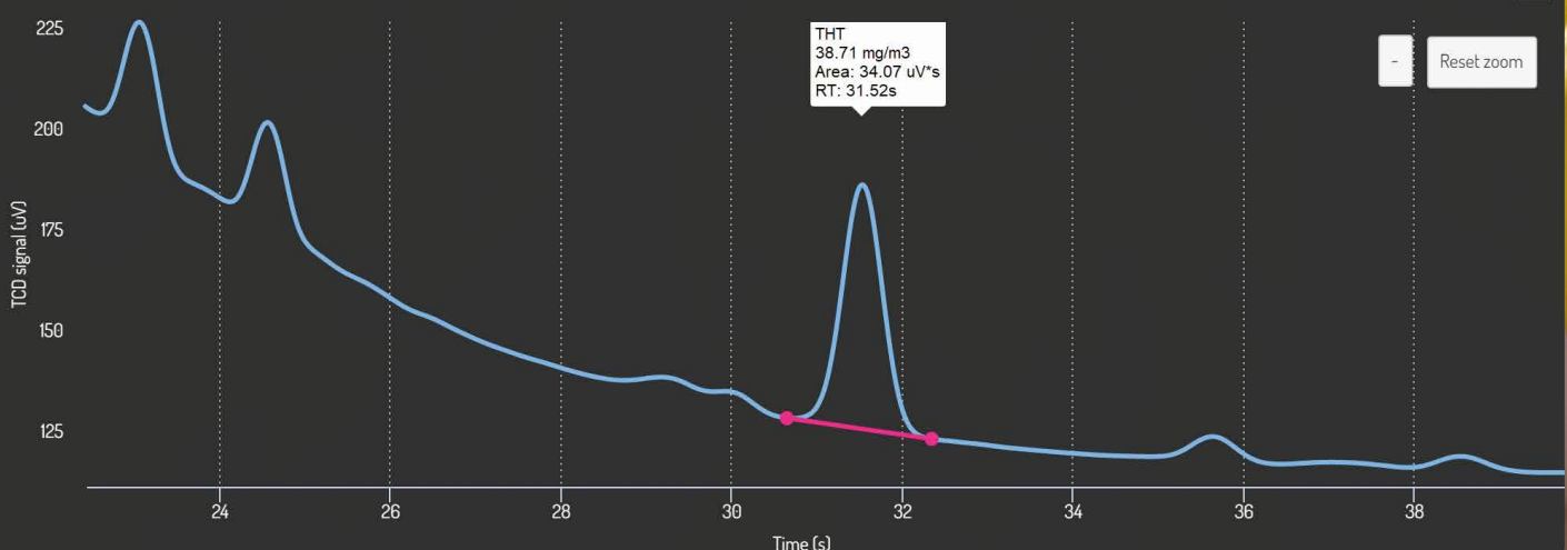
CHROMATOGRAM
